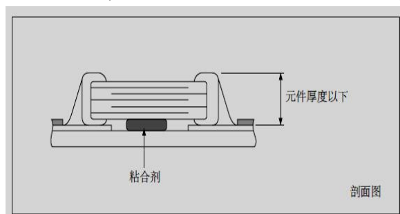
The optimal solder fillet amounts for wave soldering
